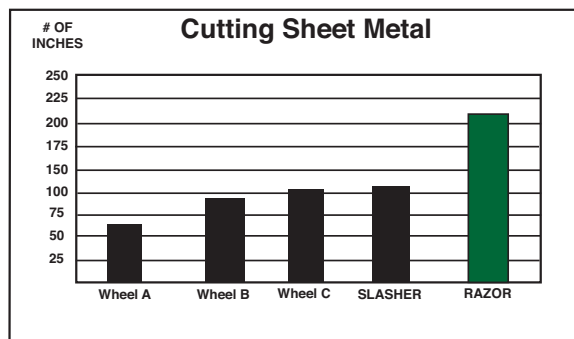
3" X 1/32" X 3/8" A/O Wheels tested on 20 ga steel
