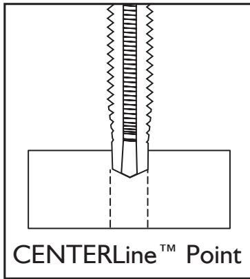
Plug-Tap Point
