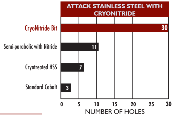
Test block is 316 Stainless Steel, thru-hole, 3/4" deep, dry cut
